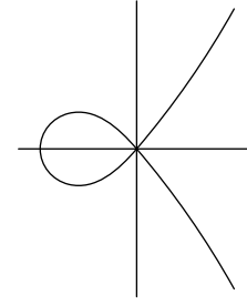
b. V(Y^2 - X^2(X + 1)) \subset \mathbb{A}^2
